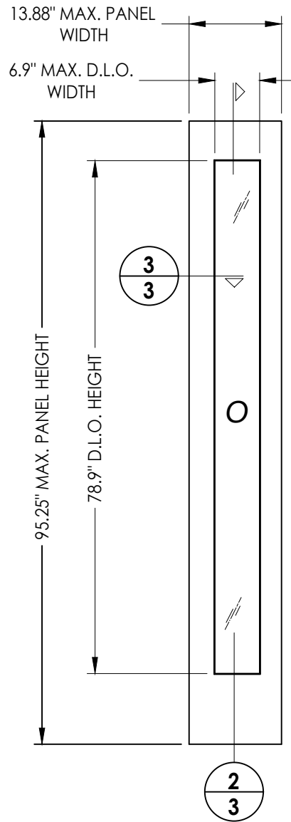
51 FIBERGLASS SIDELITE PANEL ODL
