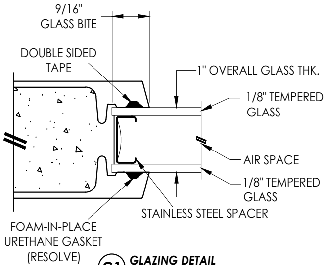
G1 GLAZING DETAIL CLEAR GLASS
