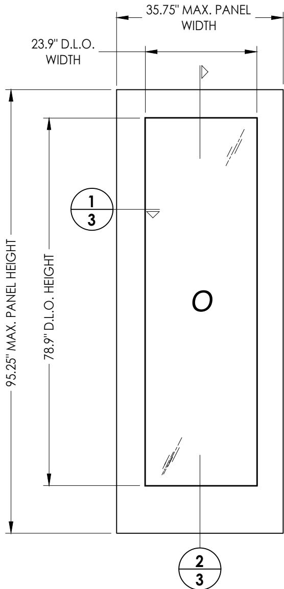
50 FIBERGLASS SIDELITE PANEL ODL FLUSH GLAZED
