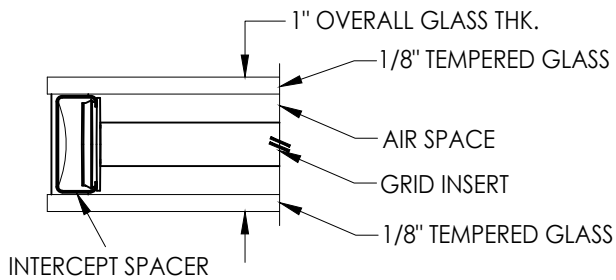
G2 GLAZING DETAIL GRIDS BETWEEN GLASS
