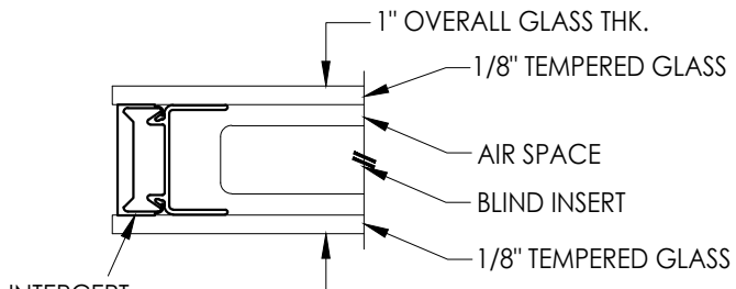
G4 GLAZING DETAIL BLINDS BETWEEN GLASS
